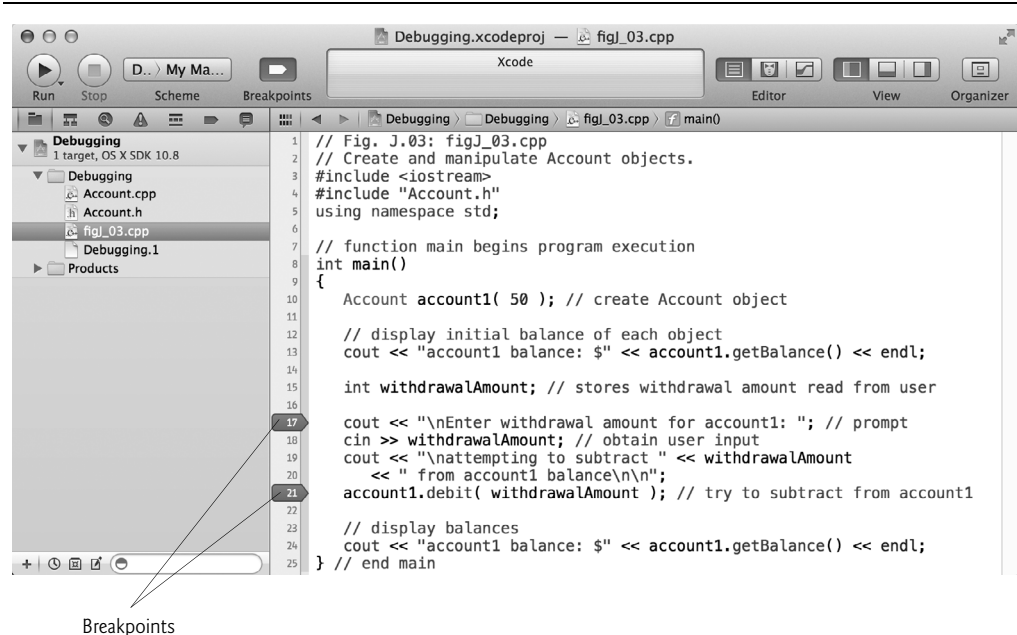
Fig. J.4 | Setting two breakpoints.
